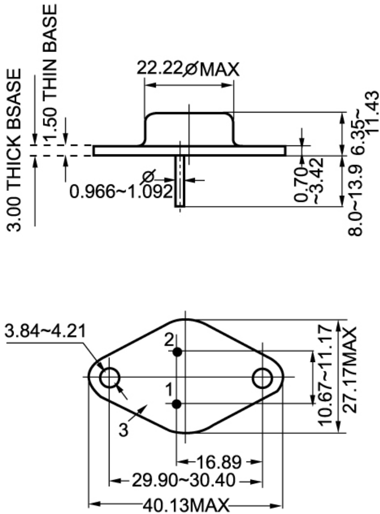
Fig.2 Outline dimensions
